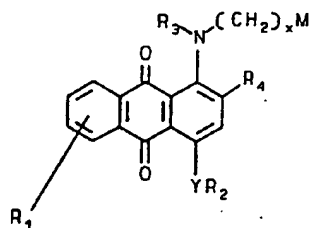
Formula II
